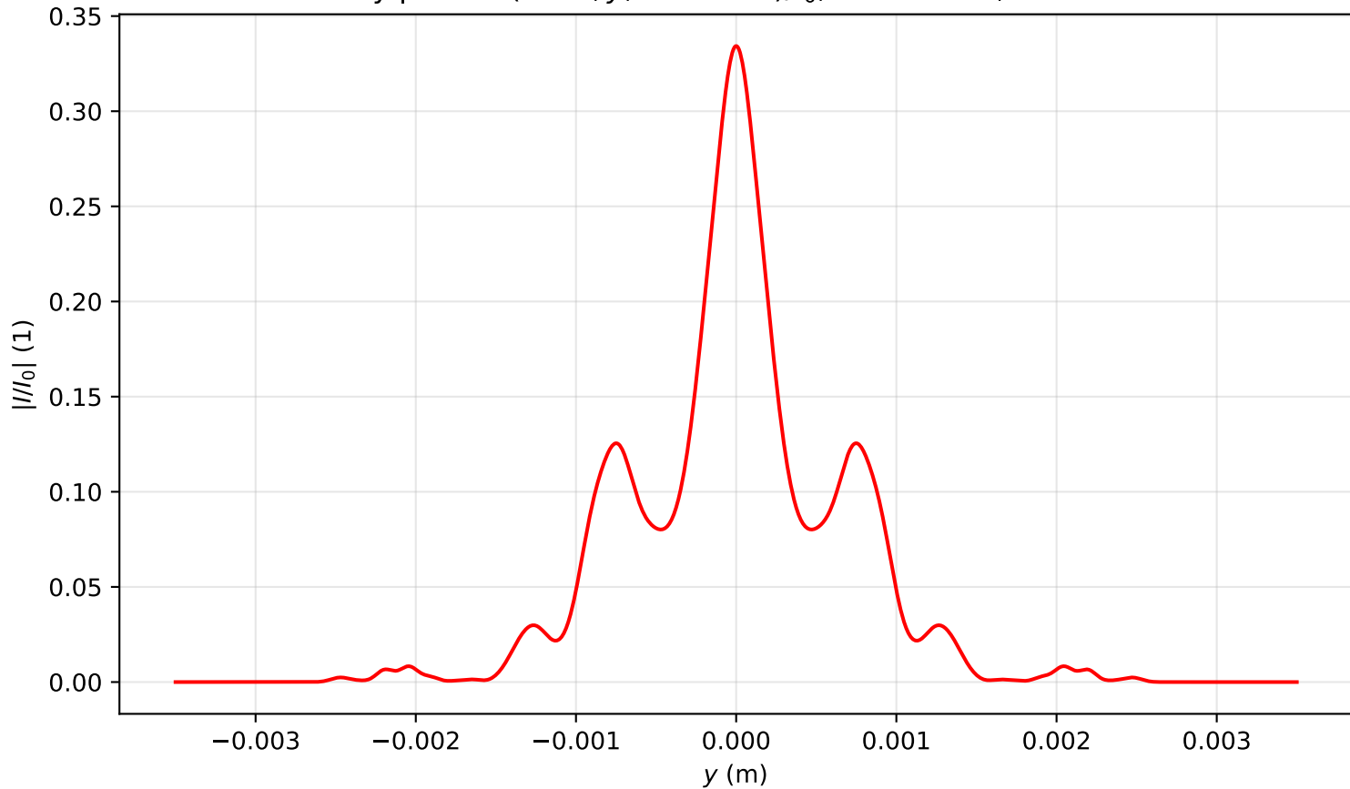
Intensity profile I(x = 0, y, z = 2.149)/I_0 , P_{in}=6.0P_{cr} , artificial time
